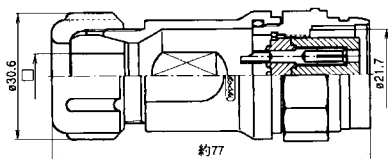
NRW-24※-AdF□
